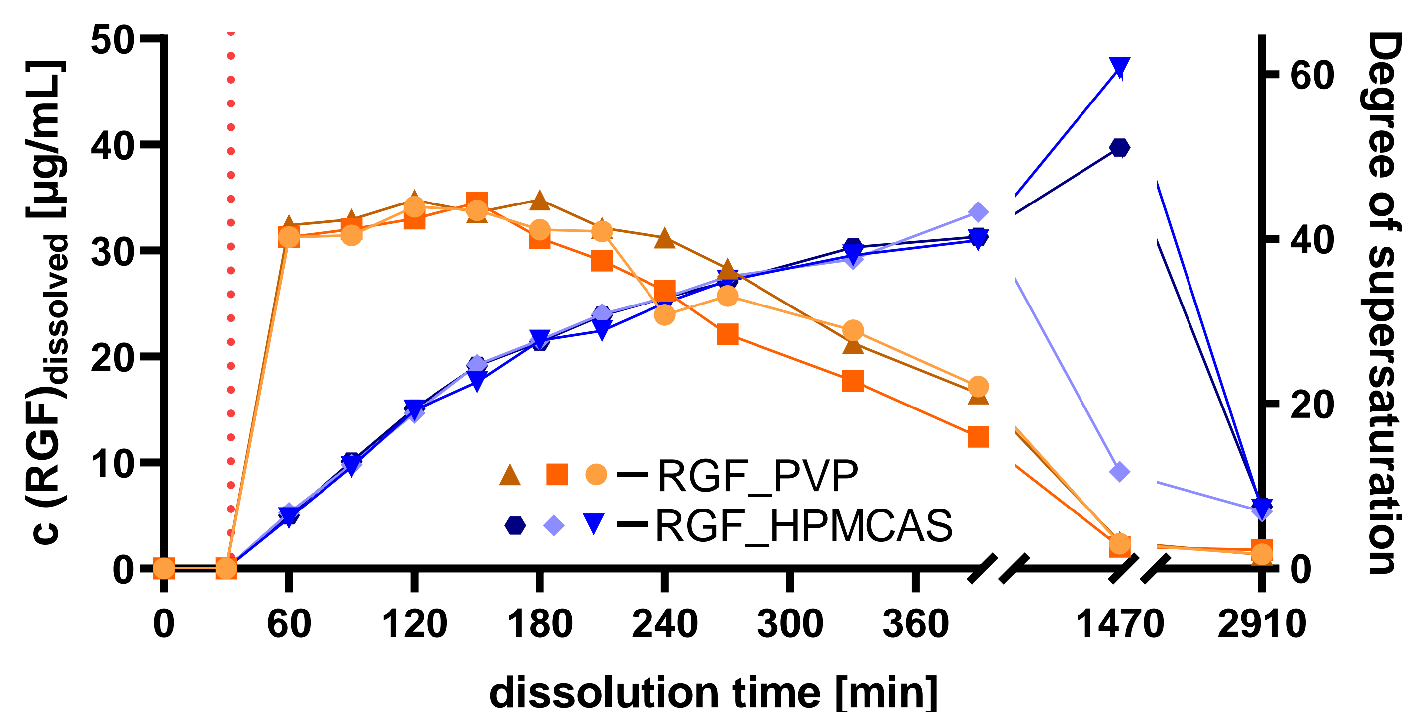
Figure 4. Two-compartment dissolution. The red line indicates the media change from FaSSGF to FaSSIF media. Single dissolution curves are shown.
