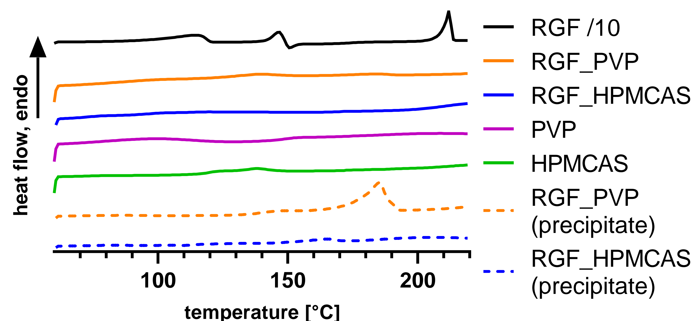
Figure 2. DSC runs of pure RGF, polymer excipients, both ASD formulations and the occurring precipitates. RGF signal was divided by 10 for illustration reasons.
